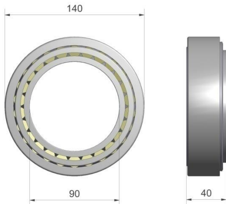
Figuur 4.3.3-Kegellager 33018
