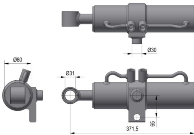
Figuur 4.2.2-Side-shift cilinder 70-30-200 Links
