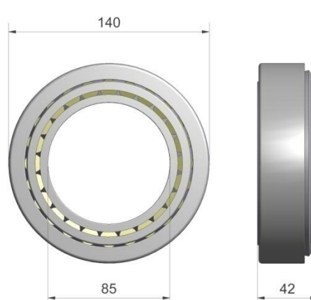
Figuur 3.3.9-Kegellager 33117
