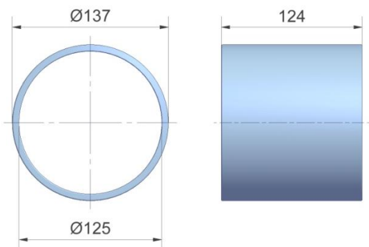
Figuur 4.3.1-D-glide lager Ø125-L124
