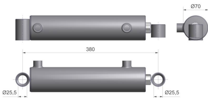
Figuur 3.2.4-Side-shift cilinder 60-30-200
