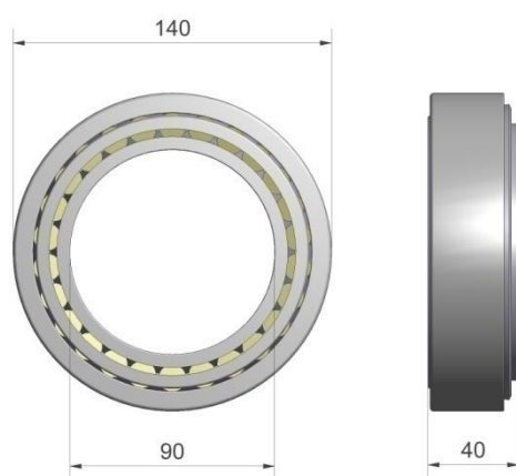
Figuur 3.3.8-Kegellager 33018
