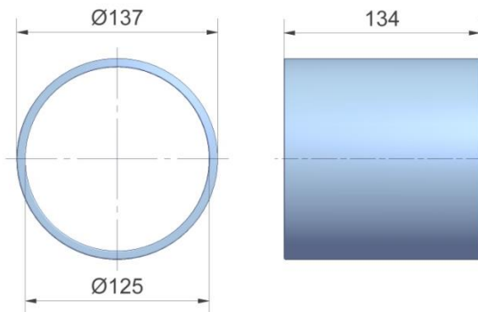
Figuur 3.3.2-D-glide lager Ø125-L134
