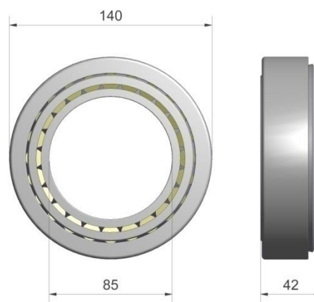
Figuur 5.2.2-Kegellager 33117
