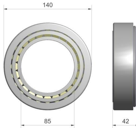
Figuur 4.3.4-Kegellager 33117
