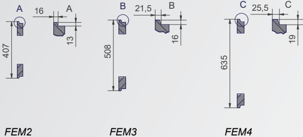
Fork carrier dimensions
