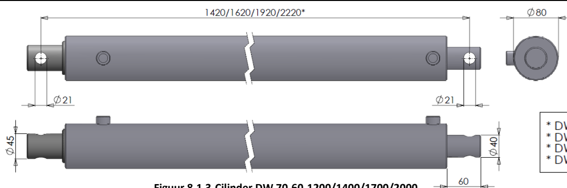
Figuur 8.1.3-Cilinder DW 70-60-1200/1400/1700/2000
