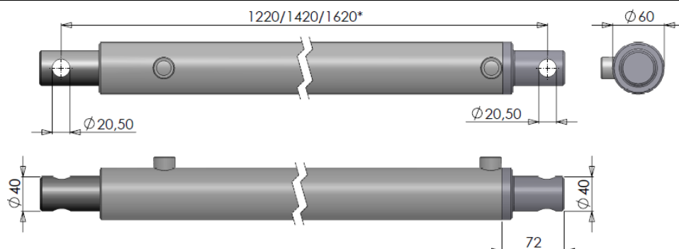
Figuur 8.1.1-Cilinder DW 50-40-1000/1200/1400
