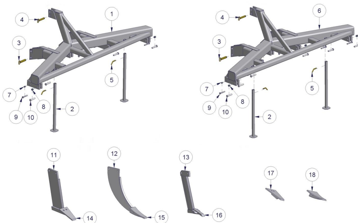
Type: WV-35
